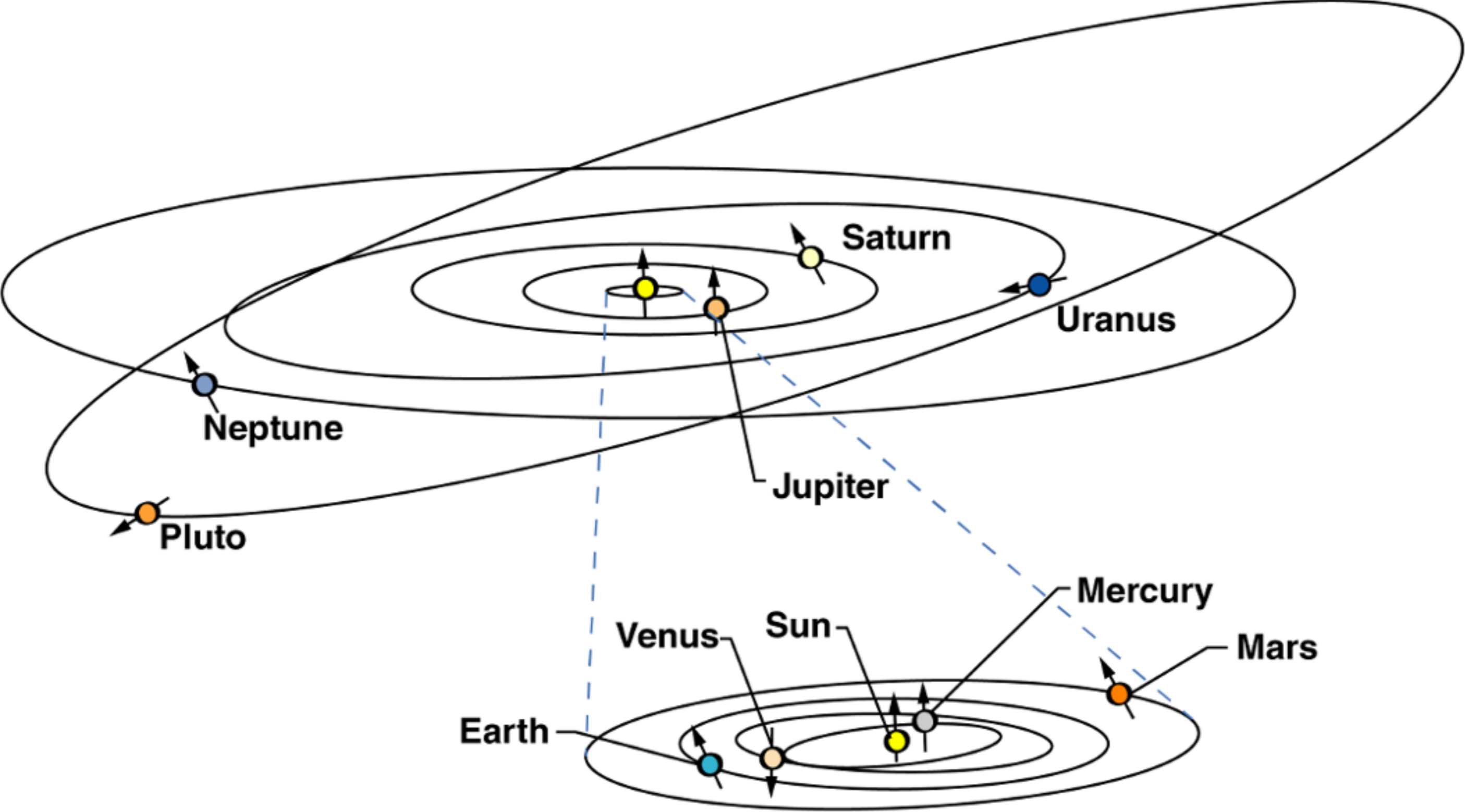
Enlargement of inner solar system
